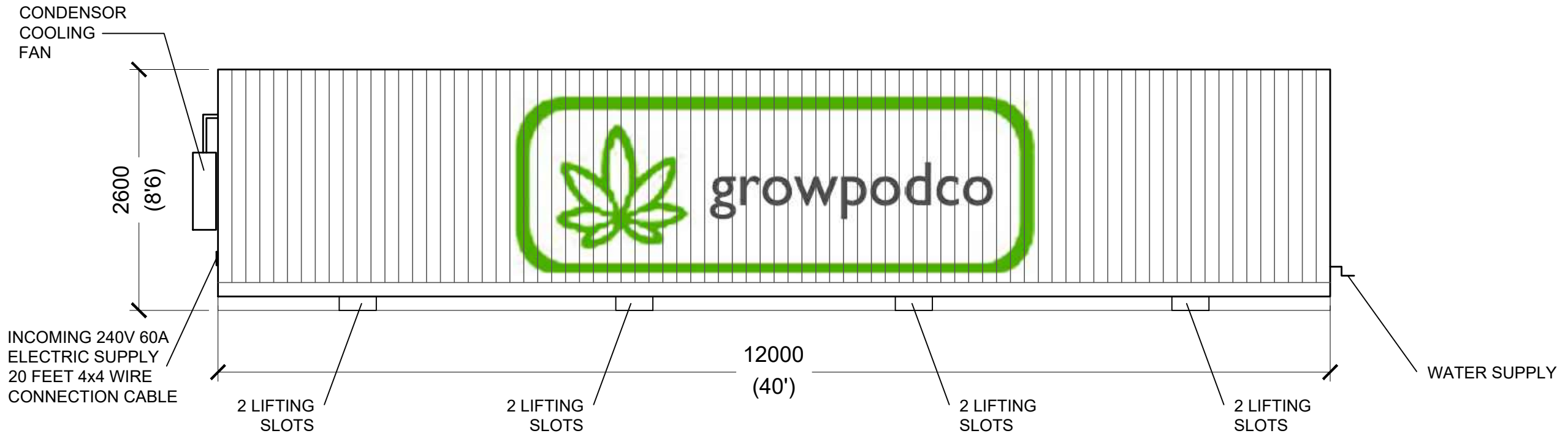
LEFT ELEVATION
